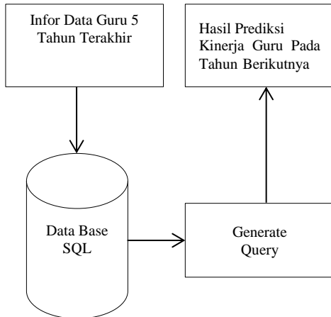
Gambar 3.1 Context Diagram
