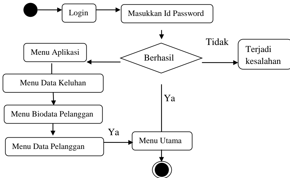
Gambar 4.4 Activity Diagram
