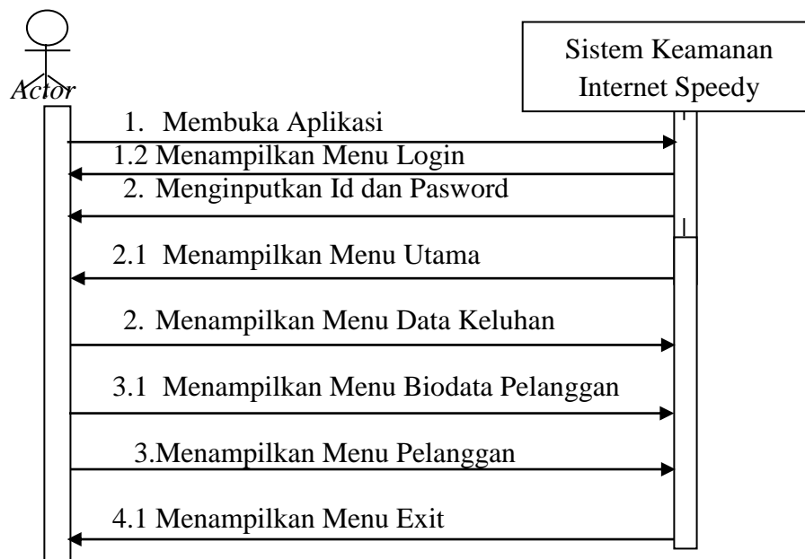
Gambar 4.3 Squence Diagram
